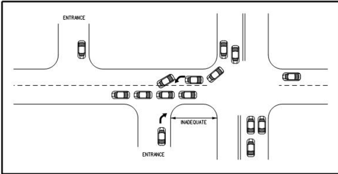
Figure 5.2.2-a Corner Clearance
