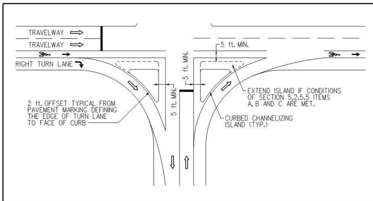
Figure 5.2.5.5-c Triangular Island Offsets
