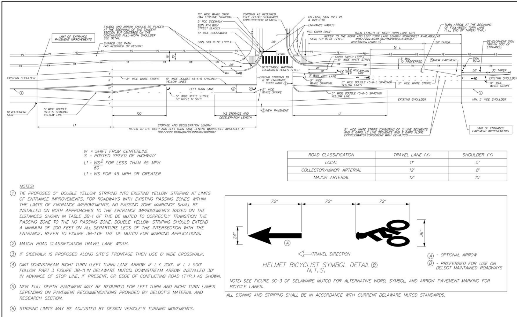
[Figure 5.2.9.3-b Typical Entrance Diagram with Left-Turn Lane]
