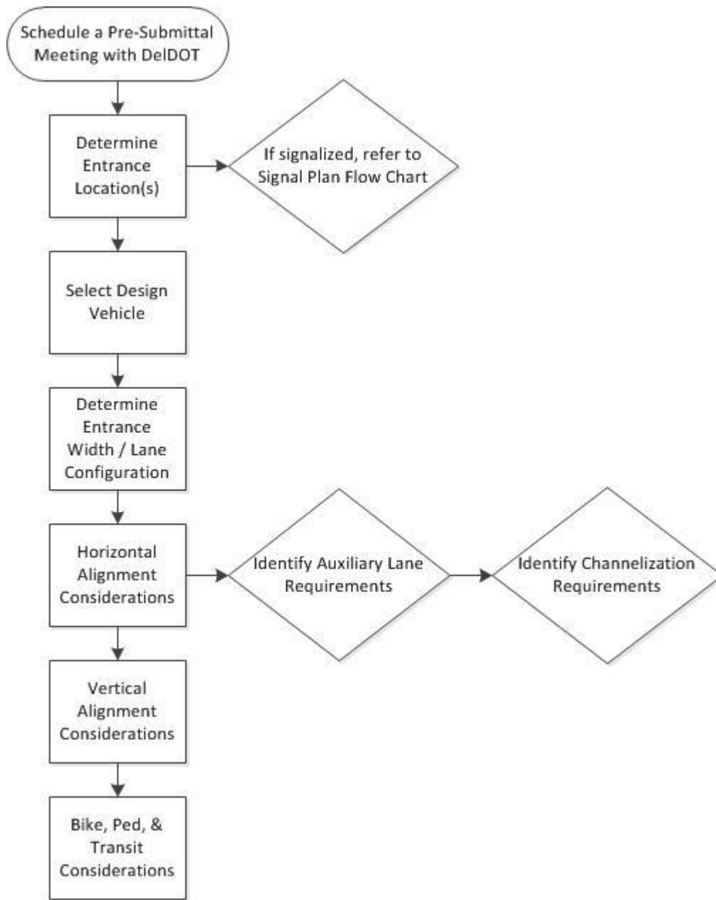
Figure 5.2.1-a Subdivision and Commercial Entrance Plan Decision Flow Chart
