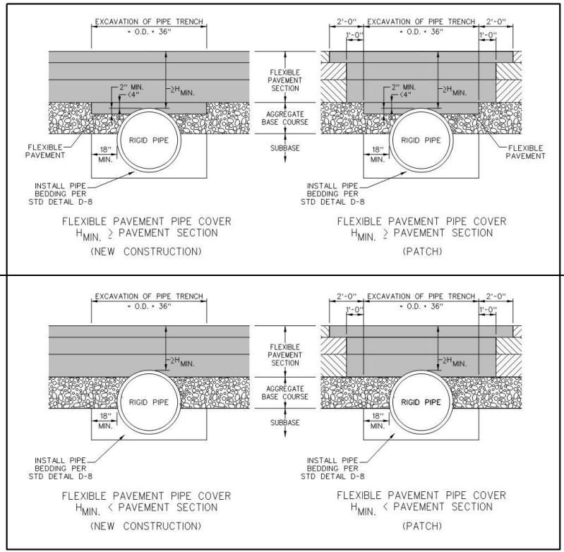
[Figure 5.7.2.5-b Existing Pavement Shallow Pipe Cover Details]
