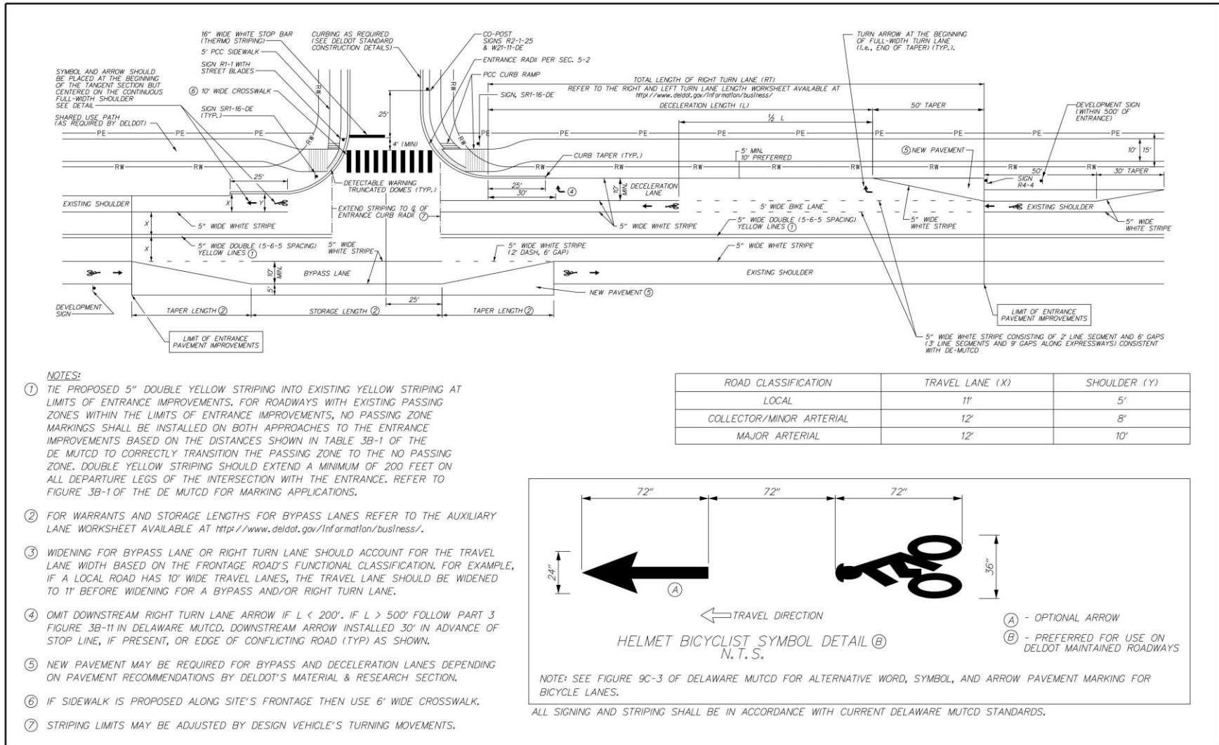
[Figure 5.2.9.2-b Typical Entrance Diagram with Bypass]
