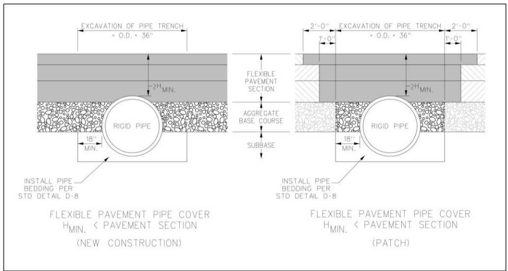
[Figure 5.7.2.5-b Existing Pavement Shallow Pipe Cover Details]
