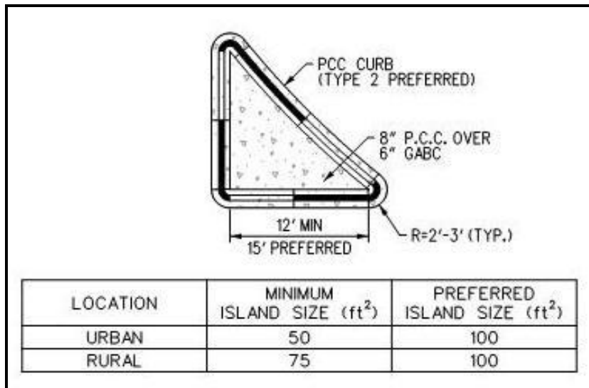
Figure 5.2.5.5-a Island Sizes without Pedestrians Facilities
