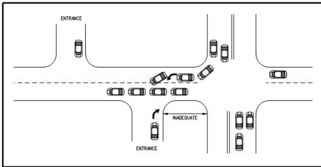
Figure 5.2.2-a Corner Clearance
