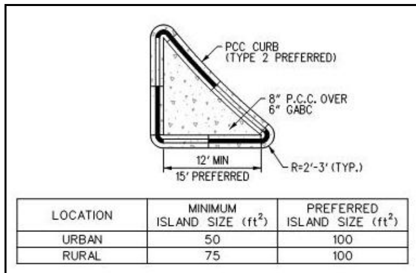
Figure 5.2.5.5-a Island Sizes without Pedestrians Facilities
