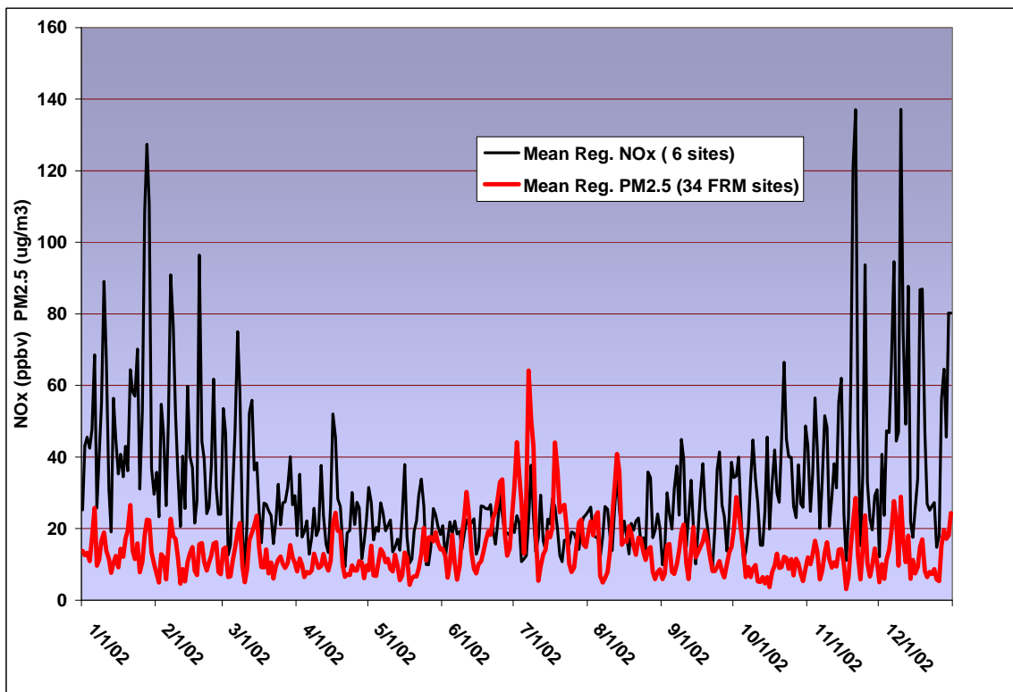
Figure C-3. Regional PM 2.5 and NO x in 2002
