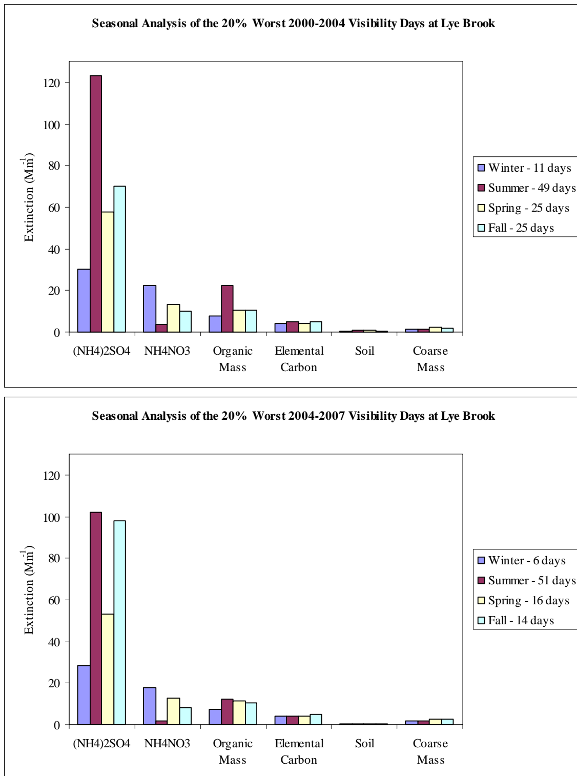
Figure 2-1. Comparison of contributions during different seasons at Lye Brook Wilderness Area on 20% worst visibility (high PM 2.5 ) days for 2000-2004 (upper) and 2004-2007 (lower)
