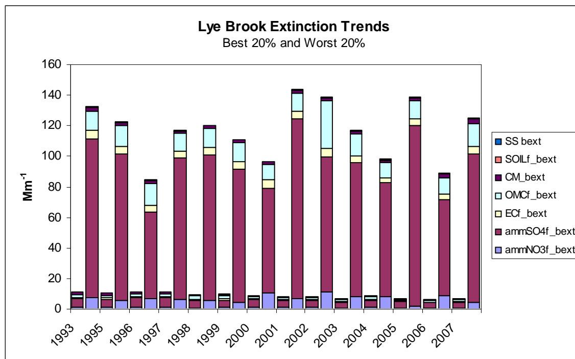
Figure 2-2. Comparison of species contributions on best and worst days at Lye Brook Wilderness Area
