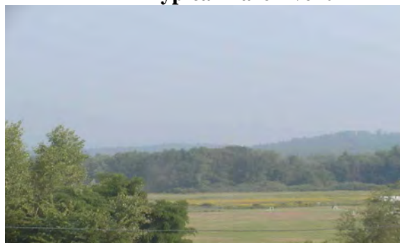
Typical Haze Event
