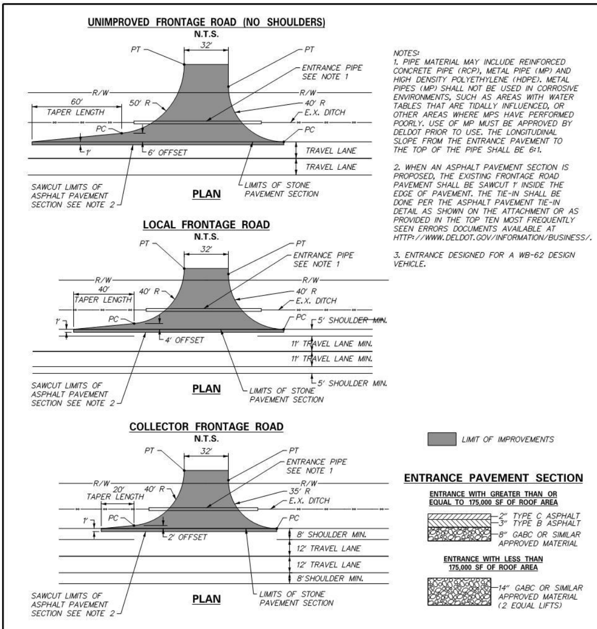
Figure 8.5.2-a Agricultural Entrance Detail
