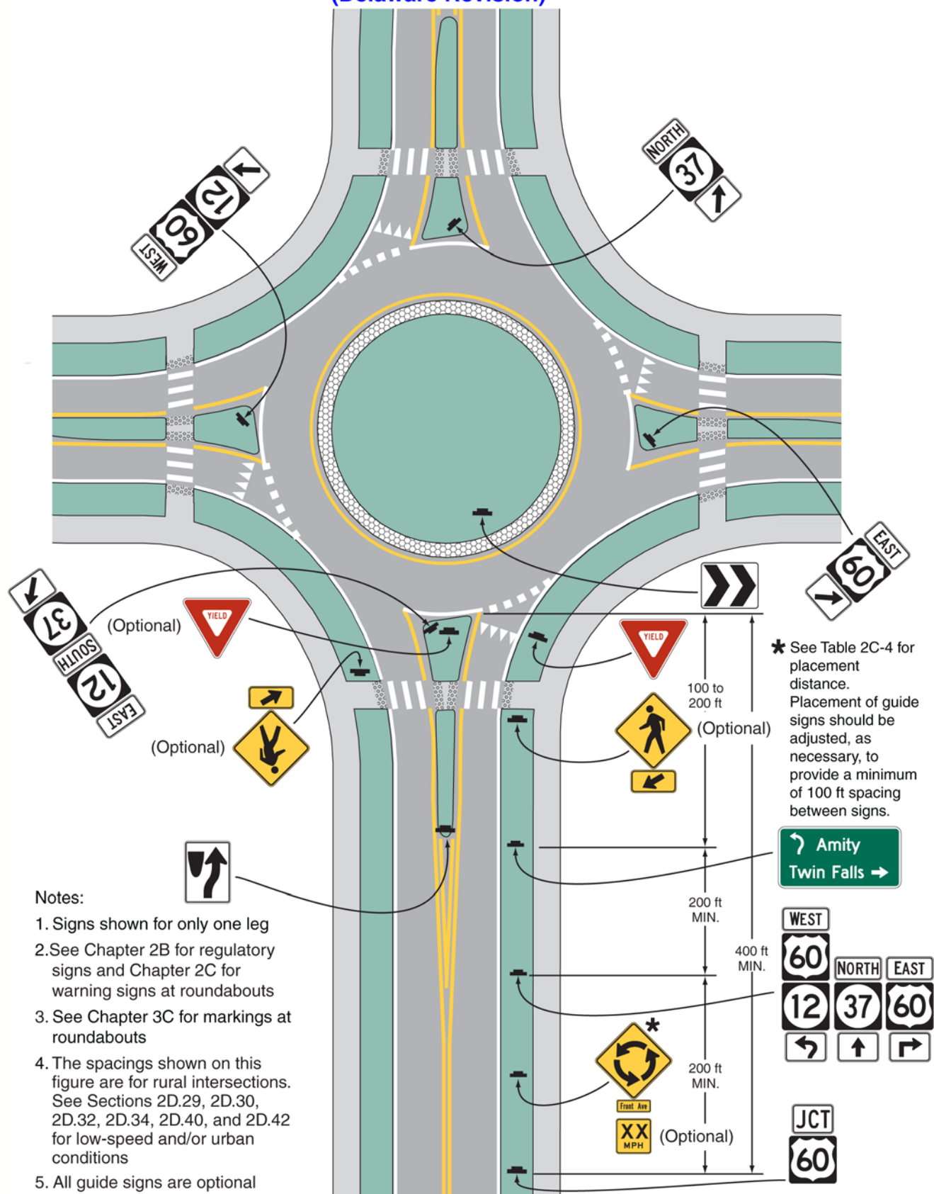
Figure 2D-9. Example of Regulatory, Warning, and Guide Signs for Roundabouts (Sheet 1 of 2)
