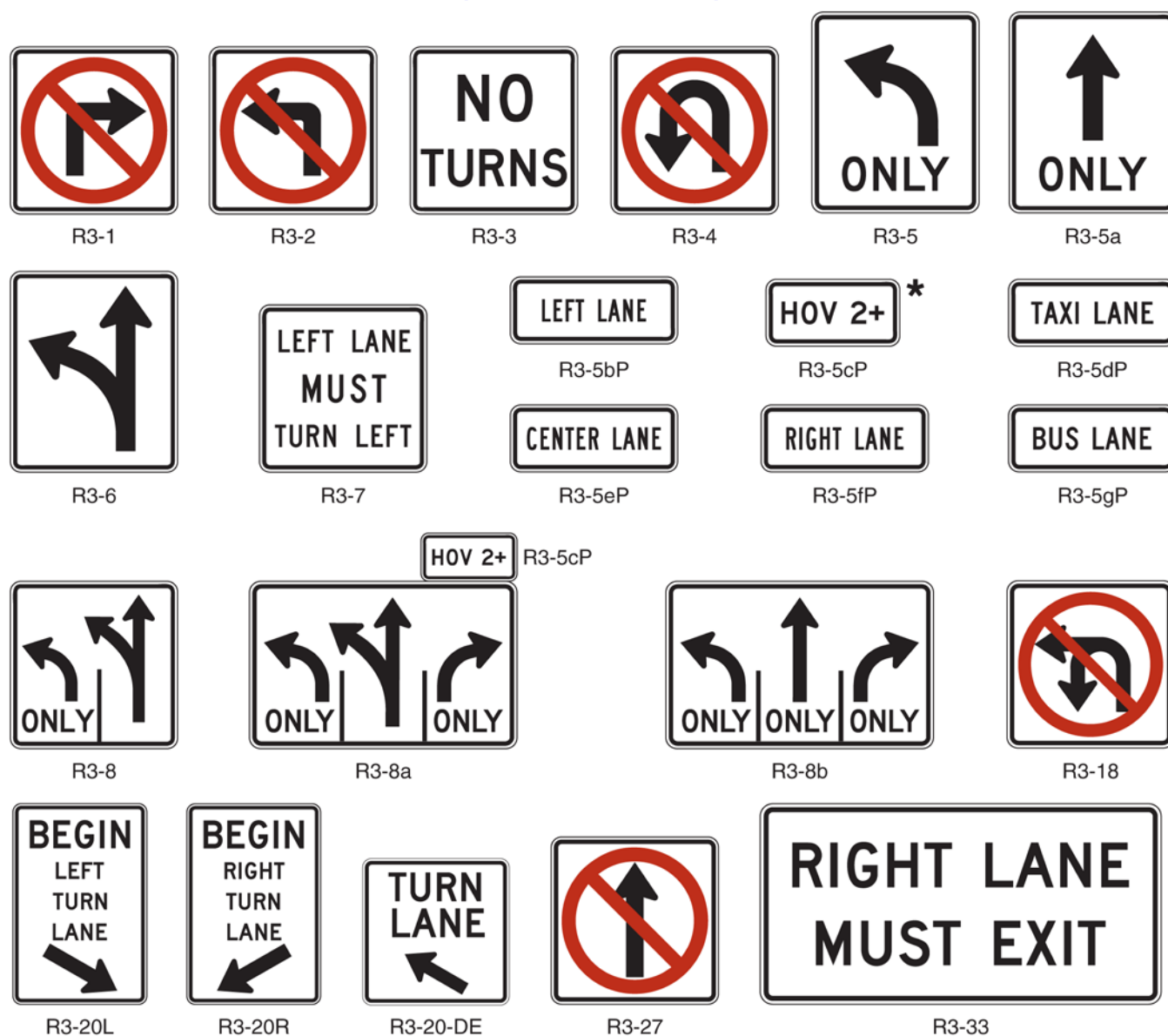
Figure 2B-4. Movement Prohibition and Lane Control Signs and Plaques (Delaware Revision)
