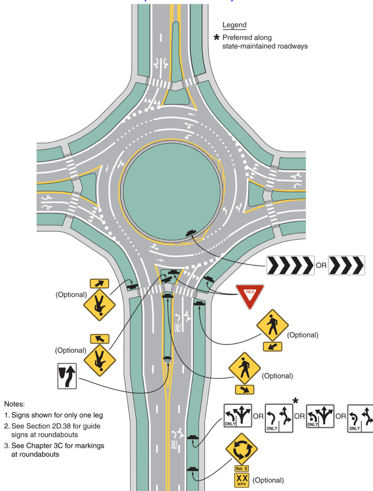
Figure 2B-23. Example of Regulatory and Warning Signs for a Two-Lane Roundabout with Consecutive Double Lefts (Delaware Revision)
