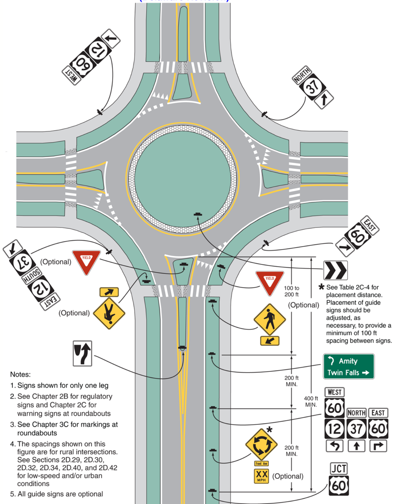
Figure 2D-9. Example of Regulatory, Warning, and Guide Signs for Roundabouts (Sheet 2 of 2)
