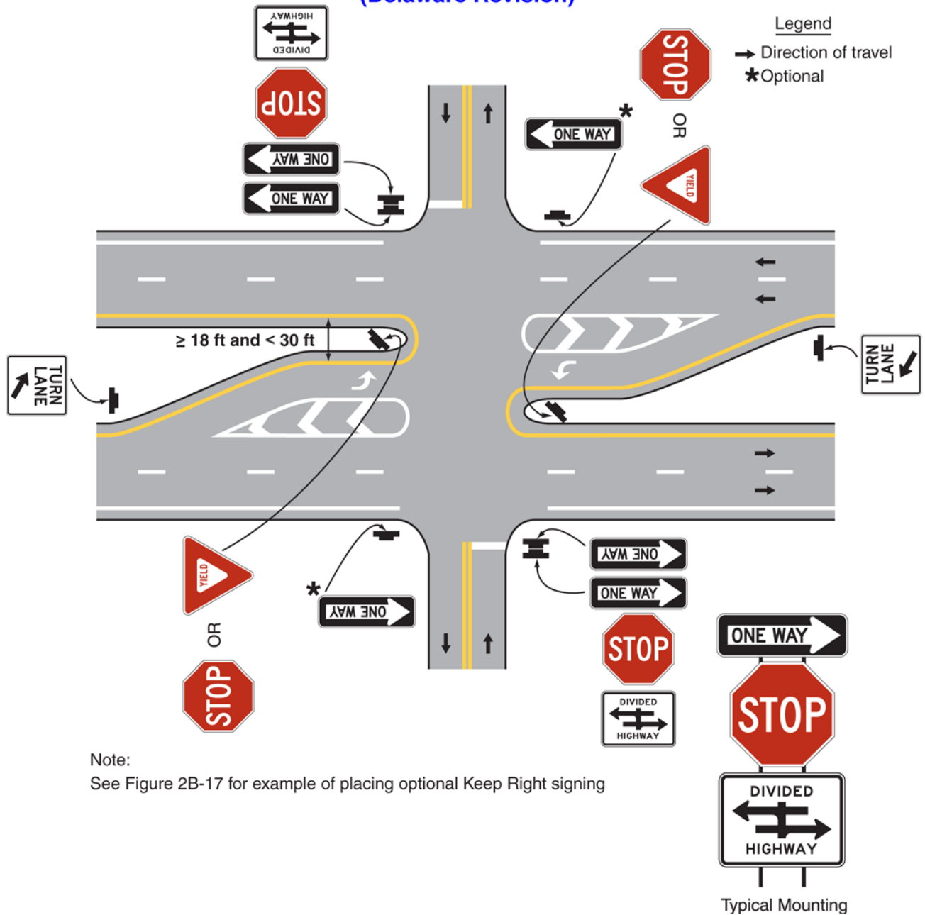
Figure 2B-17A. ONE WAY, TURN LANE, and Divided Highway Crossing Signaling for Median Openings with Separated Left-Turn Lanes along Divided Highways with Median Widths \geq 18 Feet and < 30 Feet (Delaware Revision)
