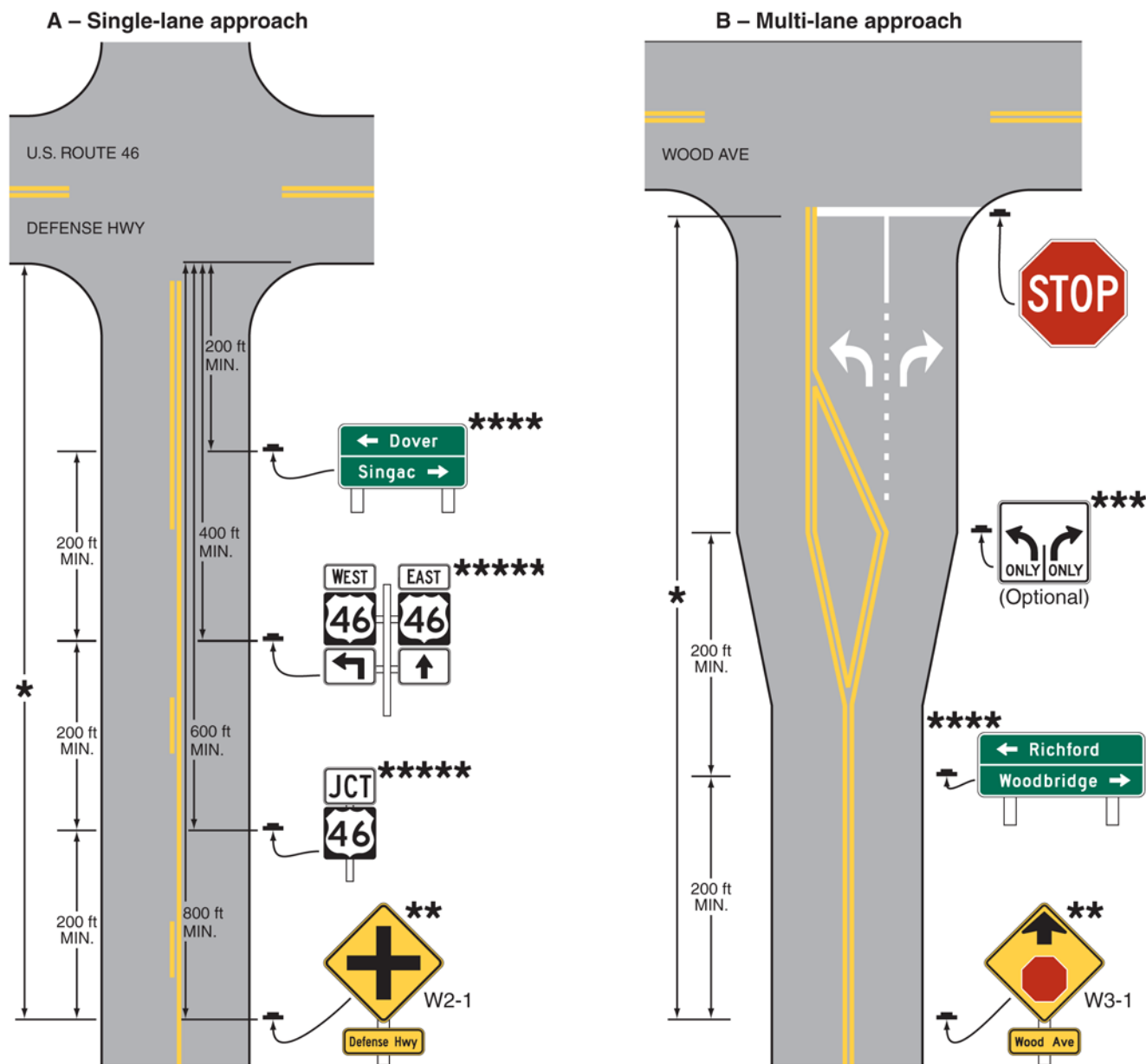
Figure 2A-4. Relative Locations of Regulatory, Warning, and Guide Signs on an Intersection Approach (Delaware Revision)
