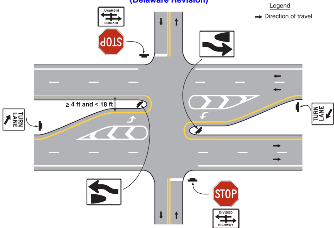
Figure 2B-17. Keep Right, TURN LANE, and Divided Highway Crossing Signing for Median Openings with Separated Left-Turn Lanes along Divided Highways with Median Widths \geq 4 Feet and < 18 Feet
