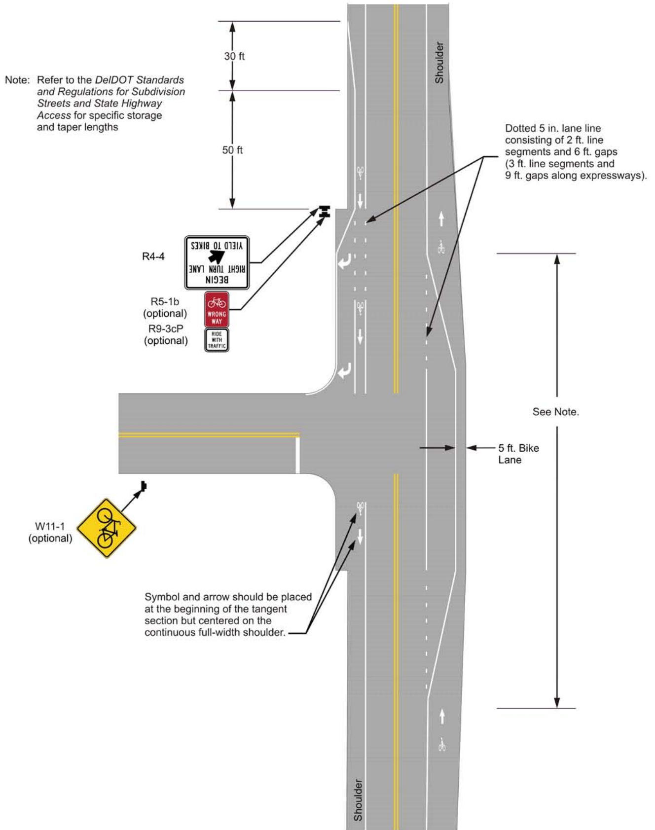
Figure 9C-1E. Example of Bicycle Lane Treatment at a Bypass Lane (Delaware Revision)
