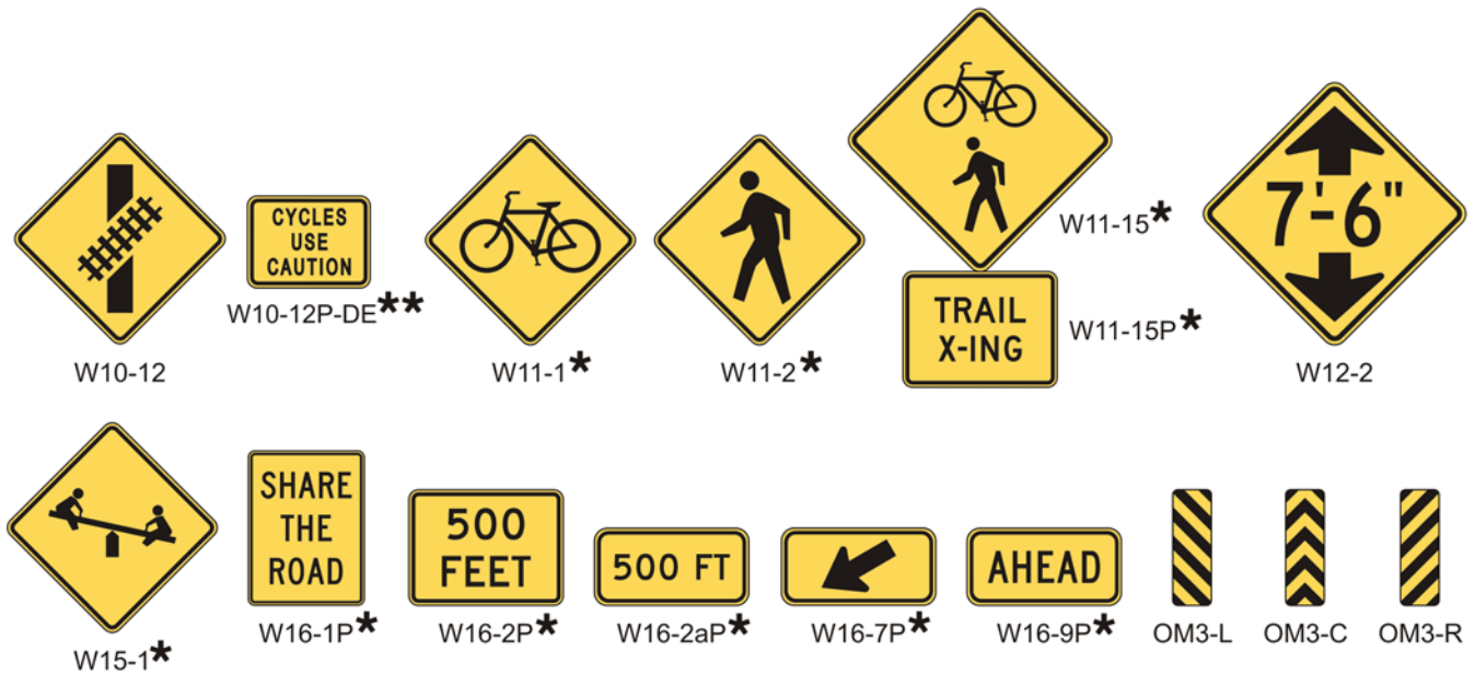
Figure 9B-3. Warning Signs and Plaques and Object Markers for Bicycle Facilities (Sheet 2 of 2) (Delaware Revision)
