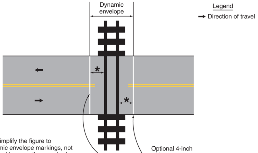
Figure 8B-8. Example of Dynamic Envelope Pavement Markings at Grade Crossings
