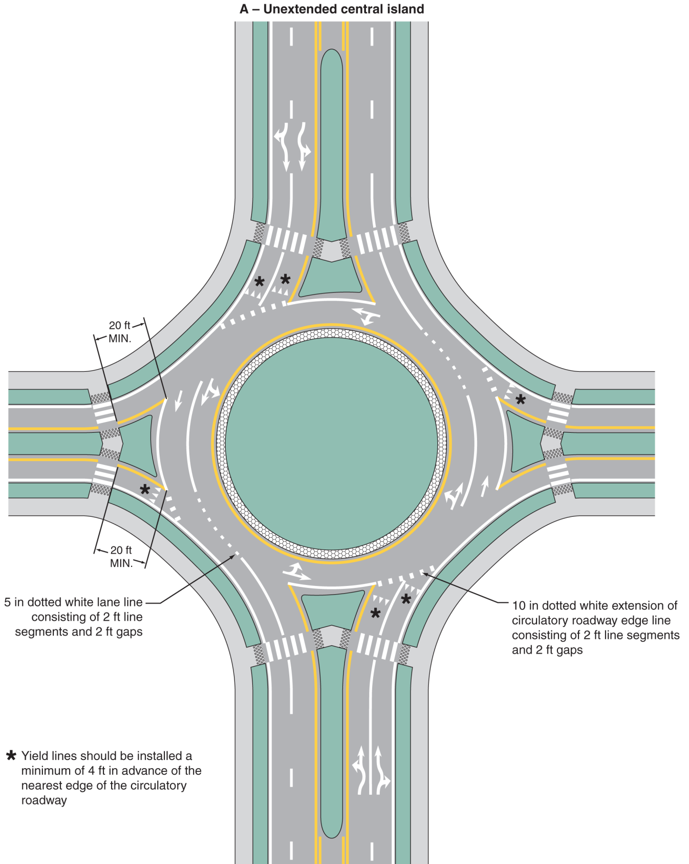
Figure 3C-4. Example of Markings for a Two-Lane Roundabout with One- and Two-Lane Approaches (Sheet 1 of 2) (Delaware Revision)
