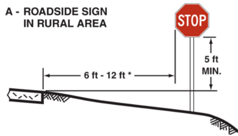
Figure 2A-2. Examples of Heights and Lateral Locations of Sign Installations (Delaware Revision)
