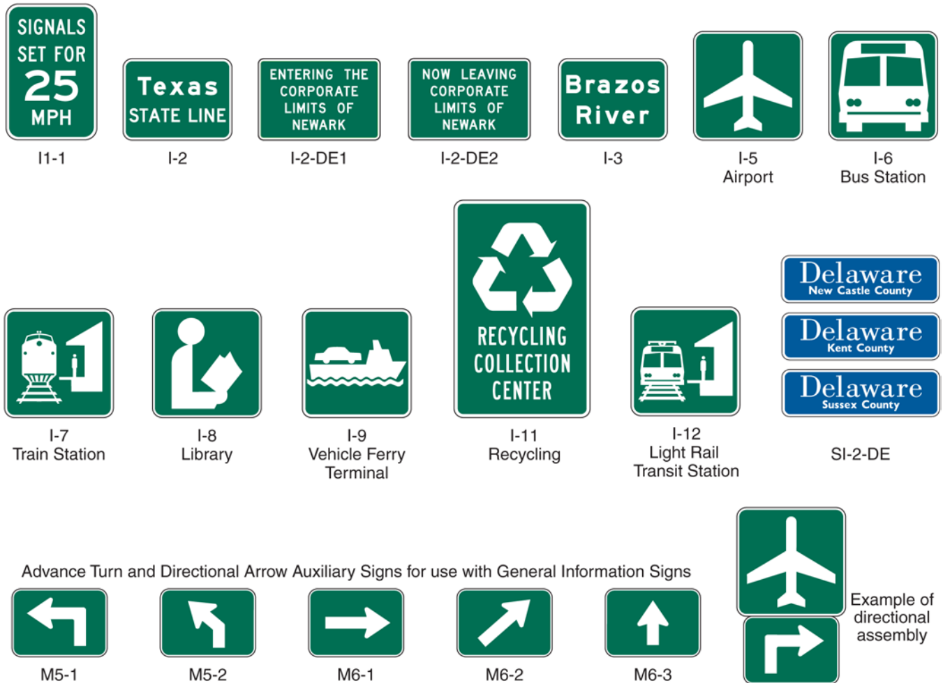
Figure 2H-1. General Information and Miscellaneous Information Signs (Delaware Revision)
