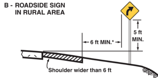
Figure 2A-2. Examples of Heights and Lateral Locations of Sign Installations (Delaware Revision)
