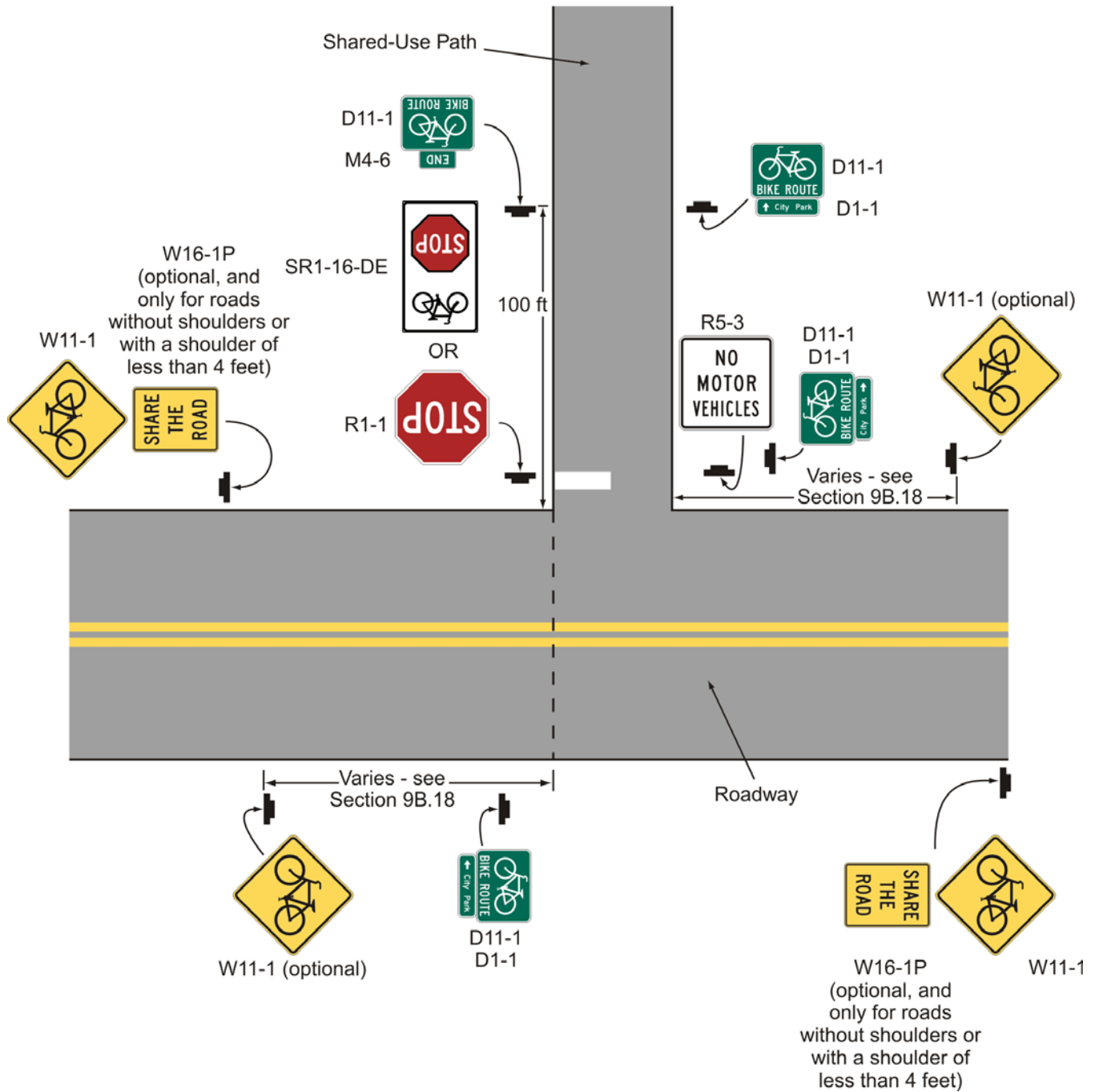
Figure 9B-5. Example of Signing for the Beginning and End of a Designated Bicycle Route (Delaware Revision)
