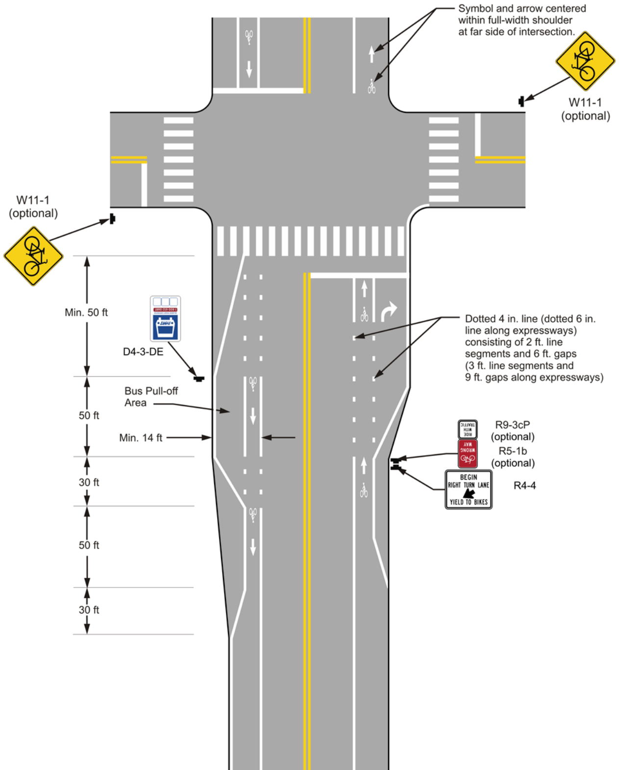
Figure 9C-6A. Example of Pavement Markings for Bicycle Lanes with Bus Pull-off Area and Full-Width Shoulder (Delaware Revision)
