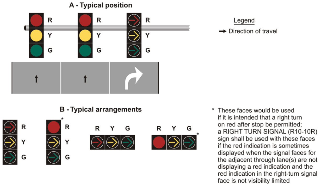
Figure 4D-17. Typical Position and Arrangements of Separate Signal Faces for Protected Only Mode Right Turns (Delaware Revision)
