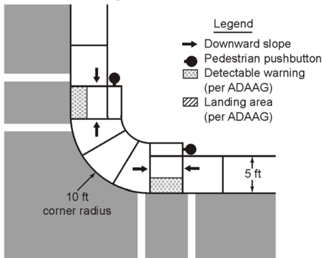
C - Parallel ramps with narrow sidewalk and tight corner radius
