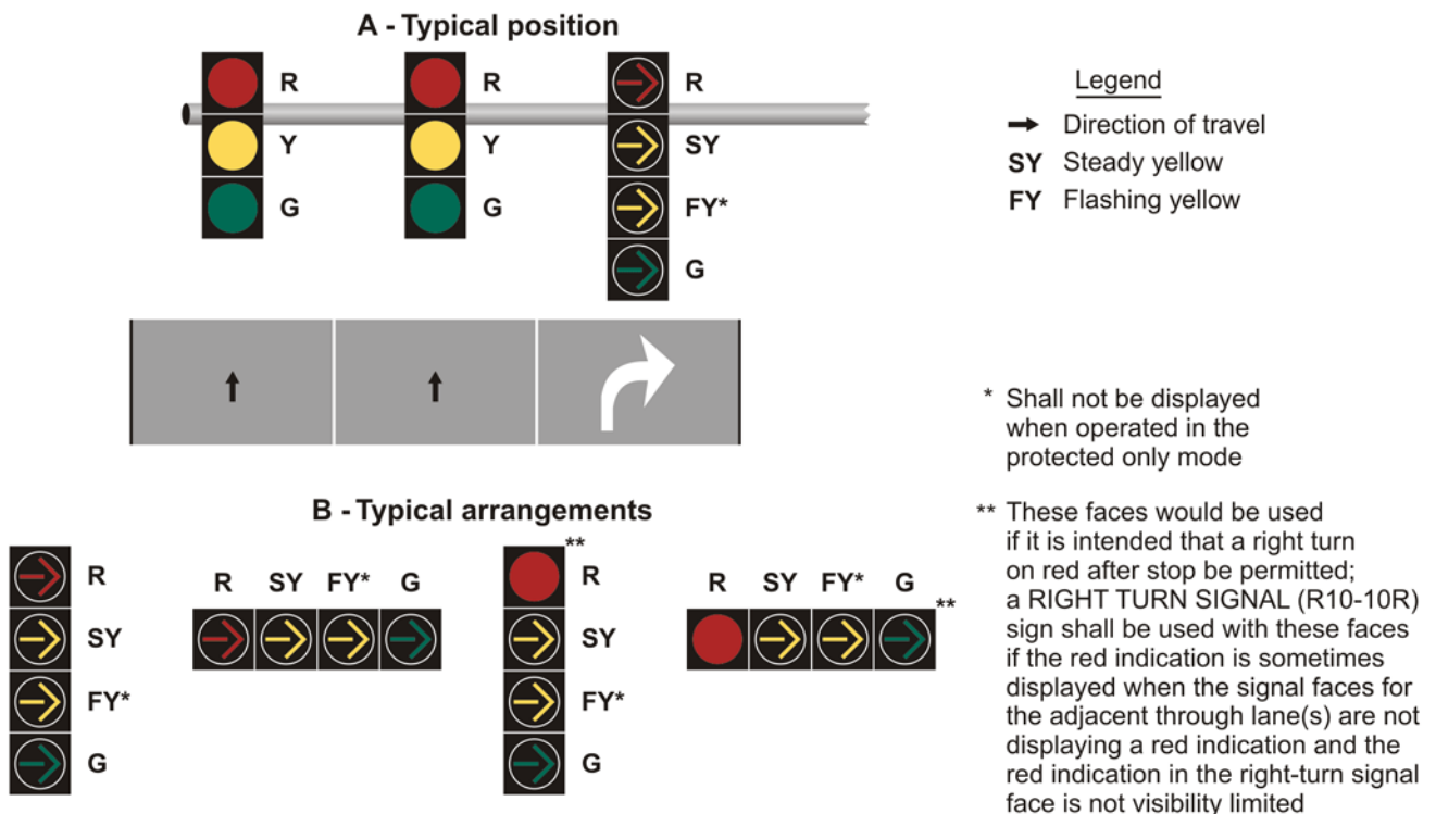
Figure 4D-19. Typical Position and Arrangements of Separate Signal Faces with Flashing Yellow Arrow for Protected/Permissive Mode and Protected Only Mode Right Turns (Delaware Revision)
