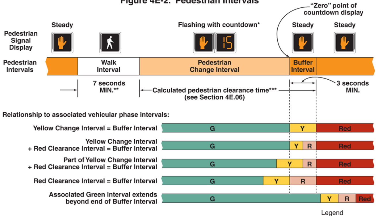
Figure 4E-2. Pedestrian Intervals
