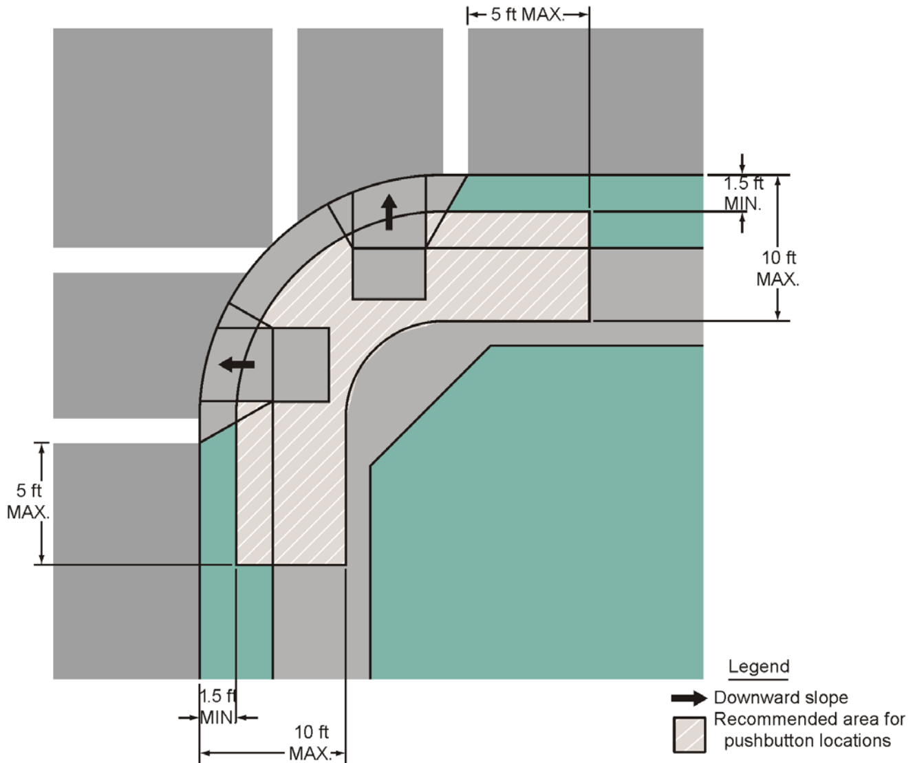
Figure 4E-3. Pushbutton Location Area (Delaware Revision)
