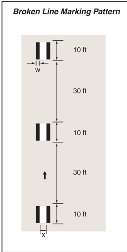
Figure 3A-1A. Black Contrast Marking Patterns on Interstates, Freeways or Expressways (Delaware Revision)
