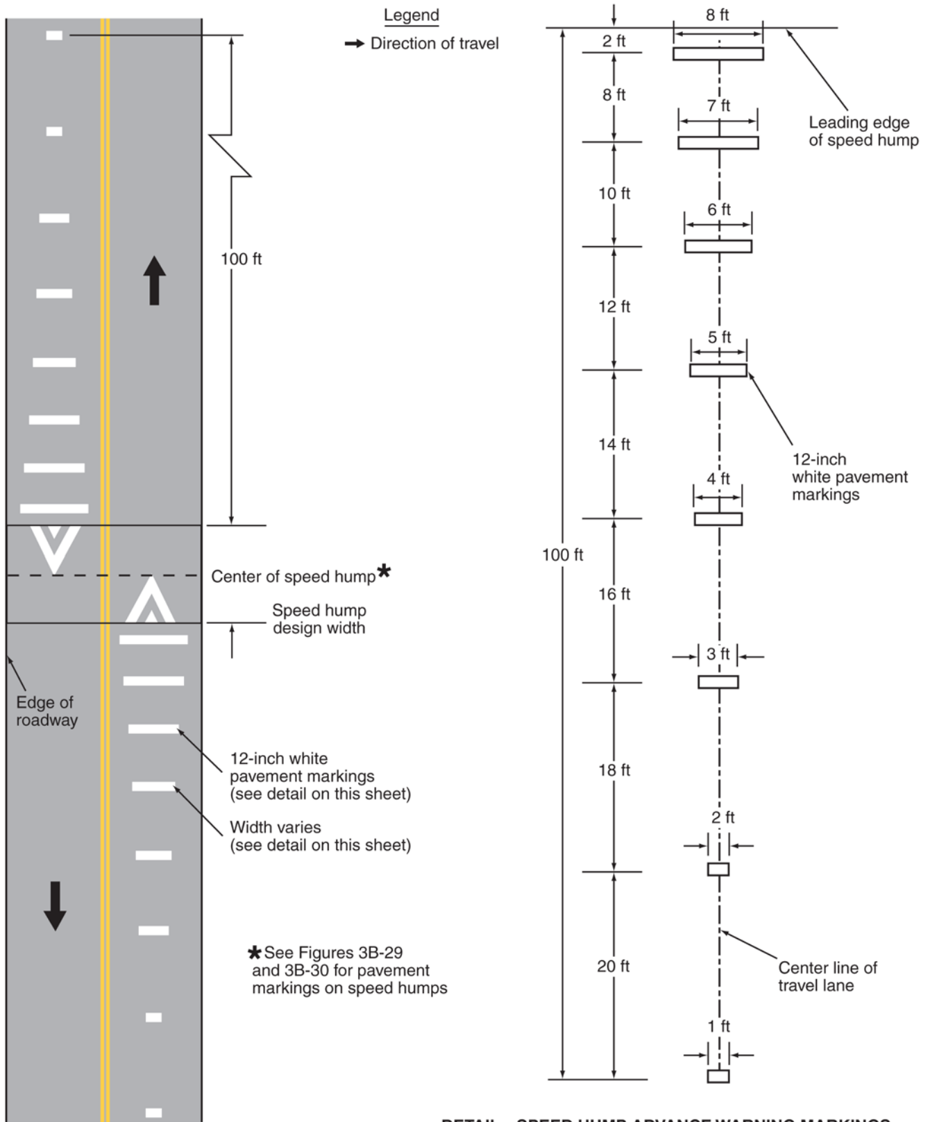
DETAIL—SPEED HUMP ADVANCE WARNING MARKINGS
