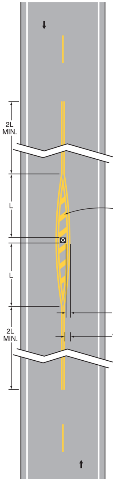
Figure 3B-15. Examples of Applications of Markings for Obstructions in the Roadway (Sheet 1 of 2) (Delaware Revision)
