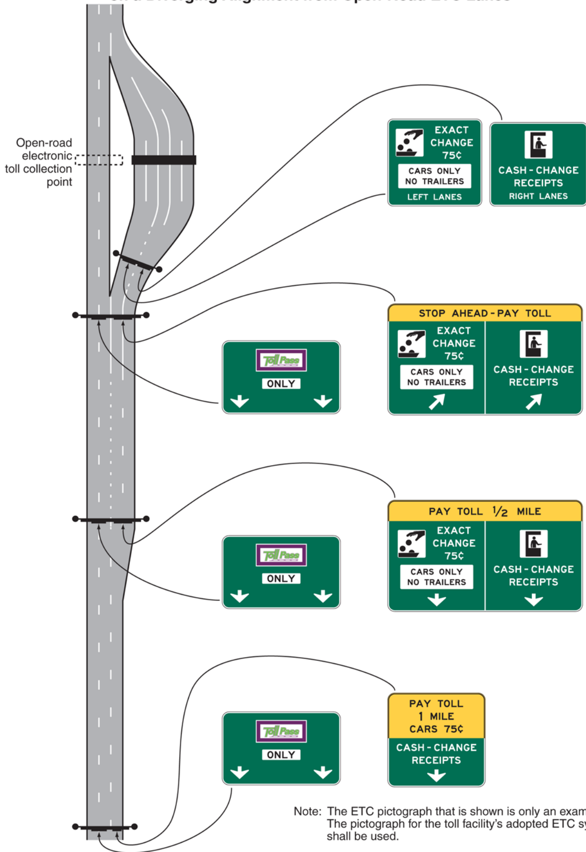
Figure 2F-11. Examples of Guide Signs for a Mainline Toll Plaza on a Diverging Alignment from Open-Road ETC Lanes
